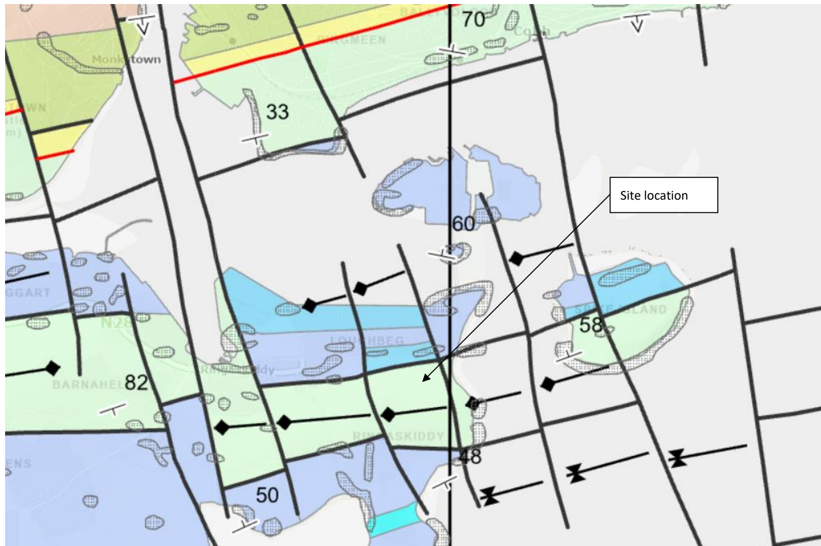
Figure 1-3: Details of the Bedrock in the Vicinity of the Indaver Site (© Geological Survey of Ireland)
